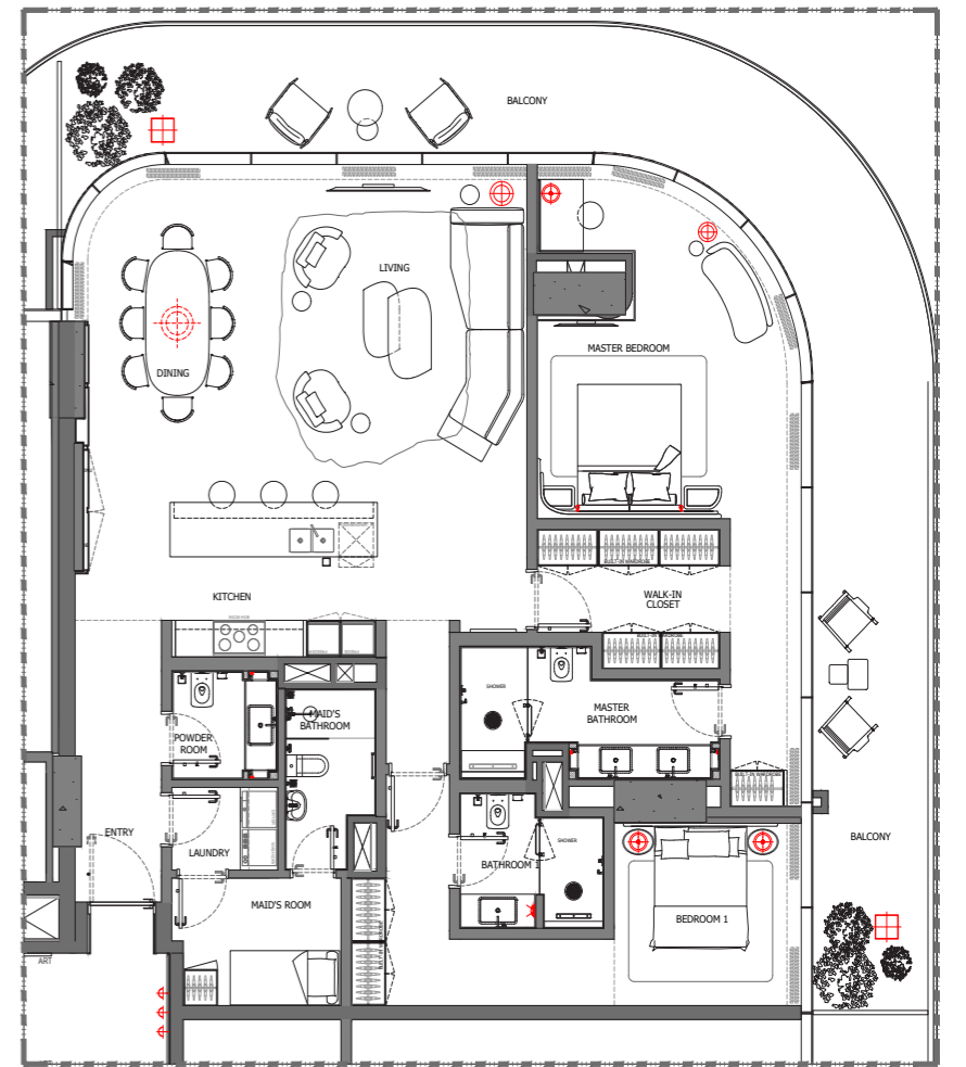
2-BR TYPE 3
