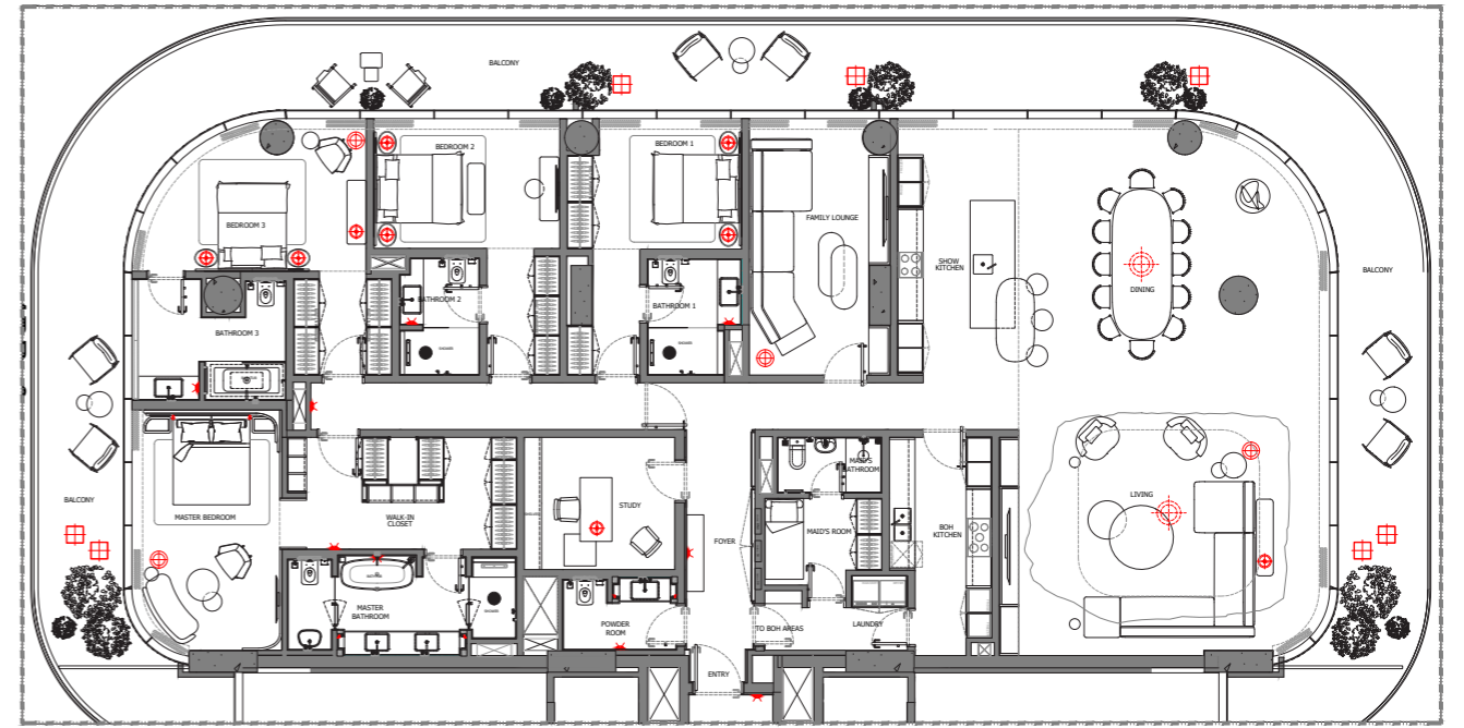
4-BR TYPE 2
